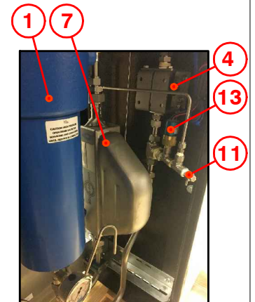
LOWER ENCLOSURE REAR RIGHT (FRONT RIGHT TYP.)
