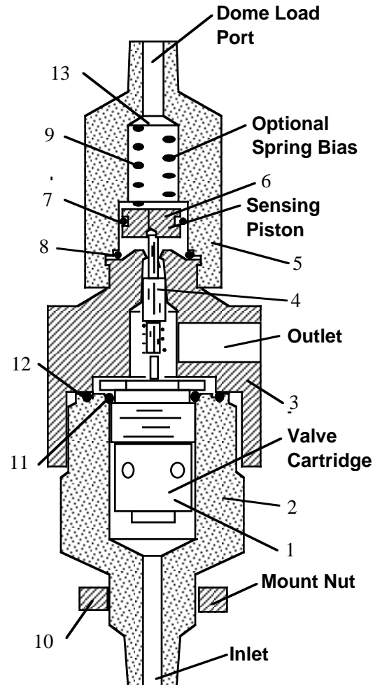
Model 1092 High Flow Dome Loading Regulator
