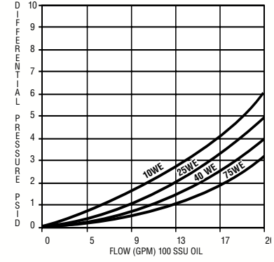
284 Stainless Elements
