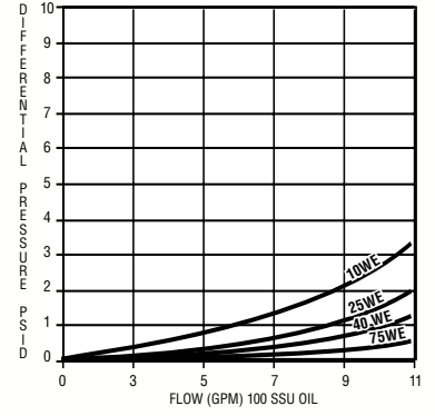
234 Stainless Elements
