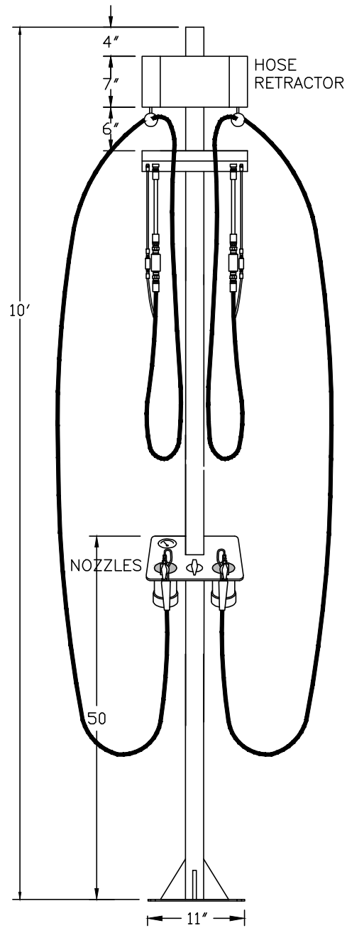
FRONT VIEW
