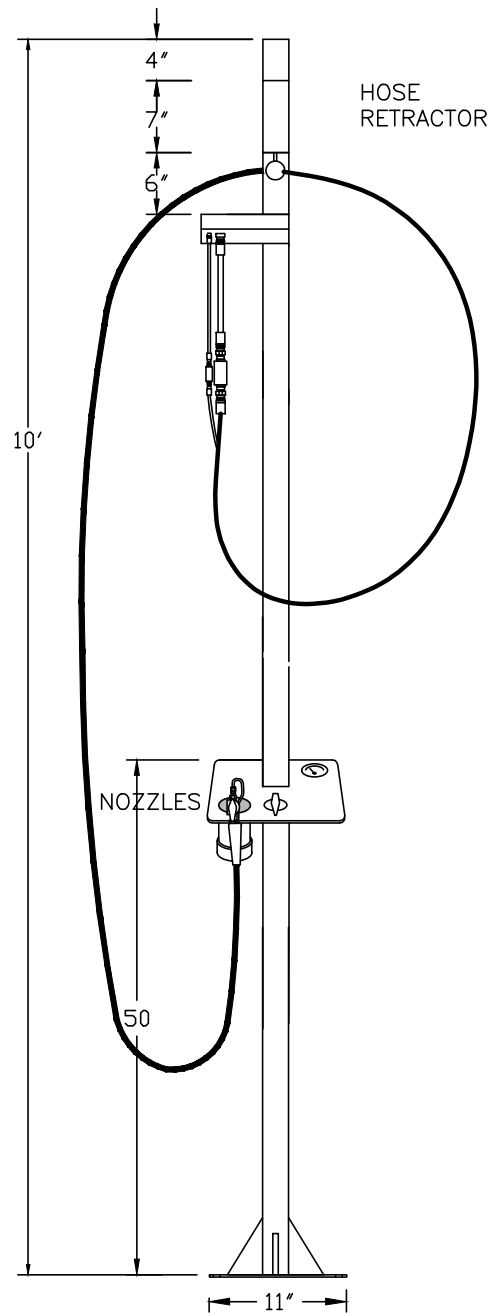
FRONT VIEW
