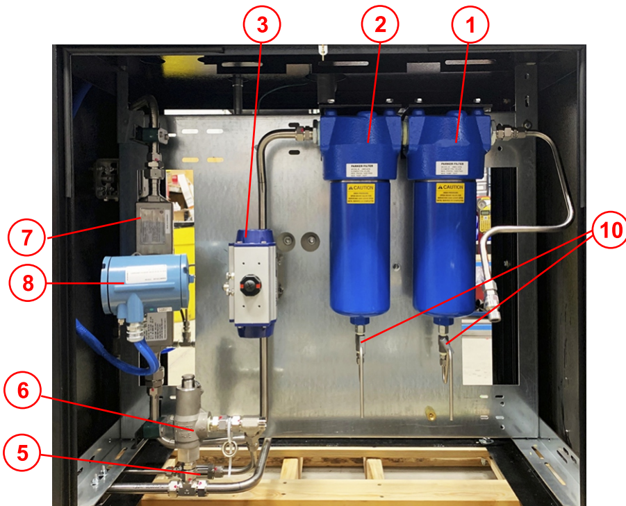
LOWER ENCLOSURE BACK
