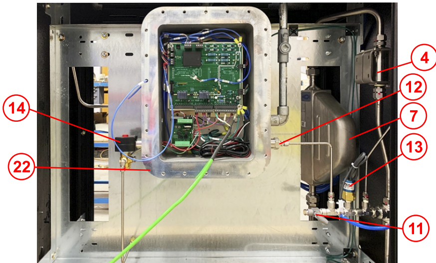
LOWER ENCLOSURE FRONT
