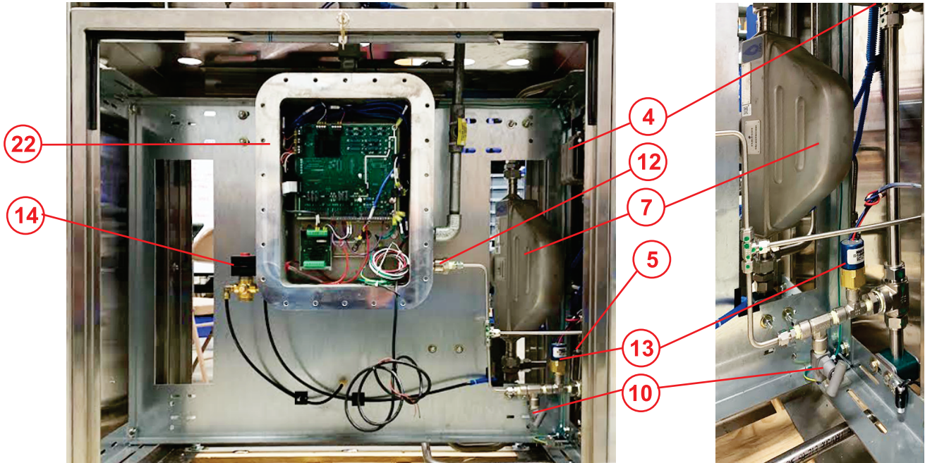
LOWER ENCLOSURE FRONT
