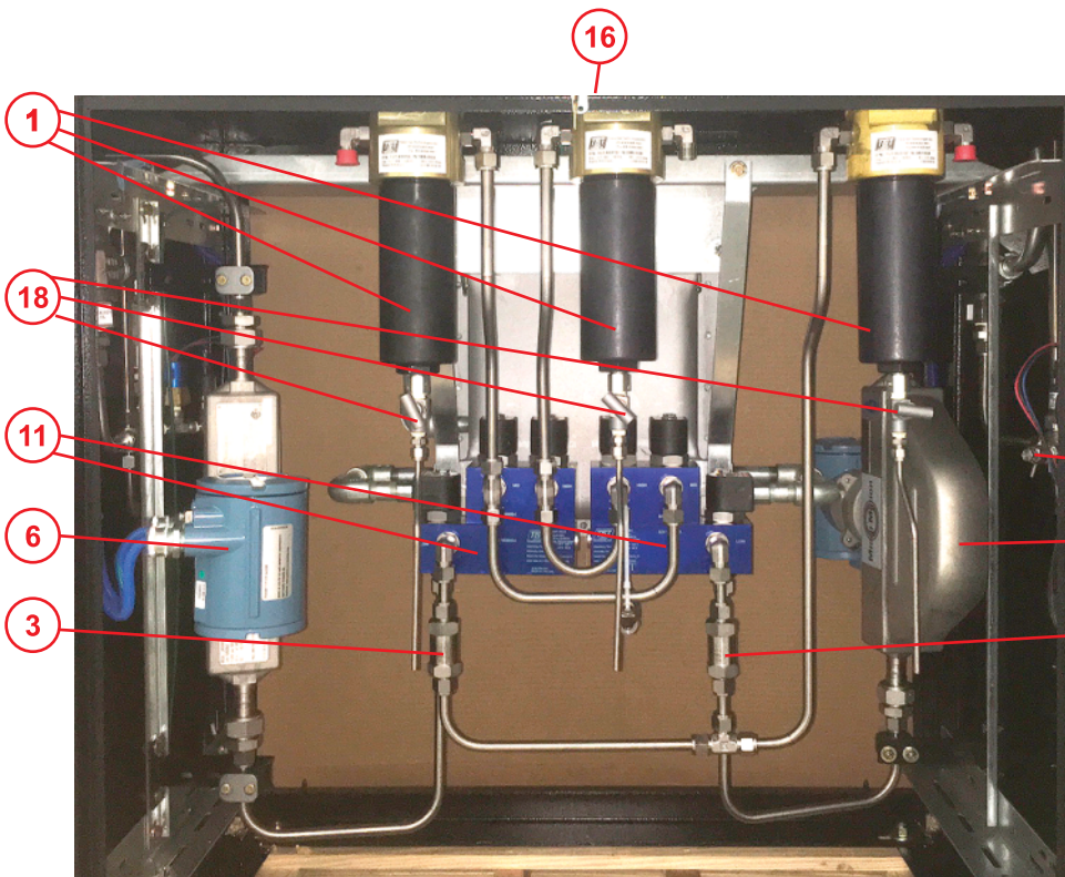
LOWER ENCLOSURE BACK
