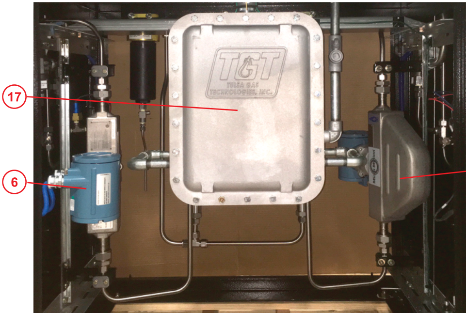
LOWER ENCLOSURE FRONT
