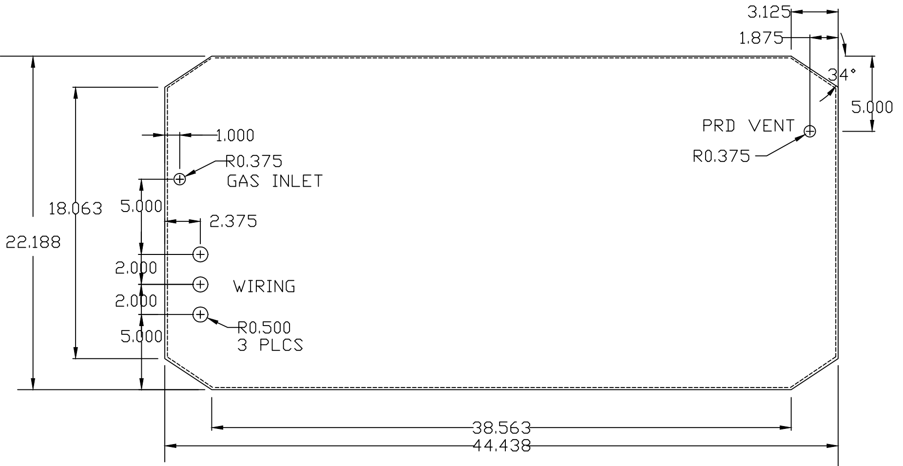
FRONT (EXPLOSION PROOF BOX SIDE)
