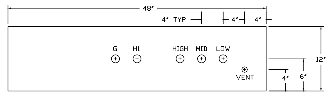
BOTTOM DETAIL
