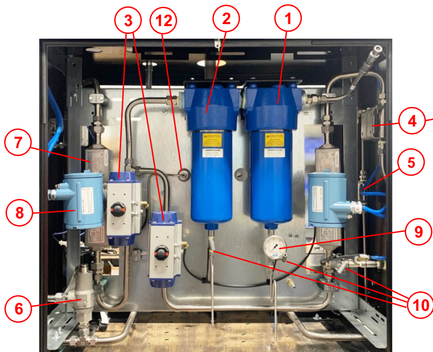
LOWER ENCLOSURE BACK
