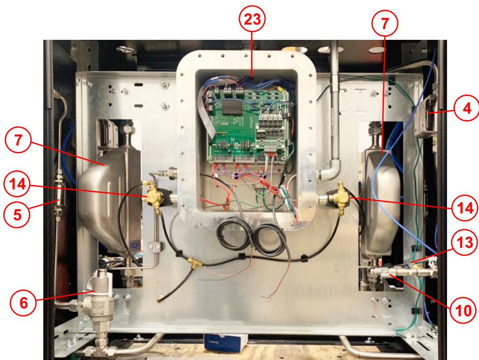
LOWER ENCLOSURE FRONT
